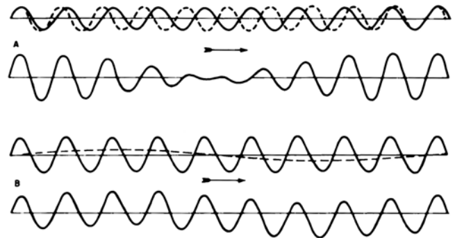
Figure 3202c. Interference. The upper part of A shows two waves of equal height and nearly equal length traveling in the same direction. The lower part of A shows the resulting wave pattern. In B similar information is shown for short waves and long swell.
