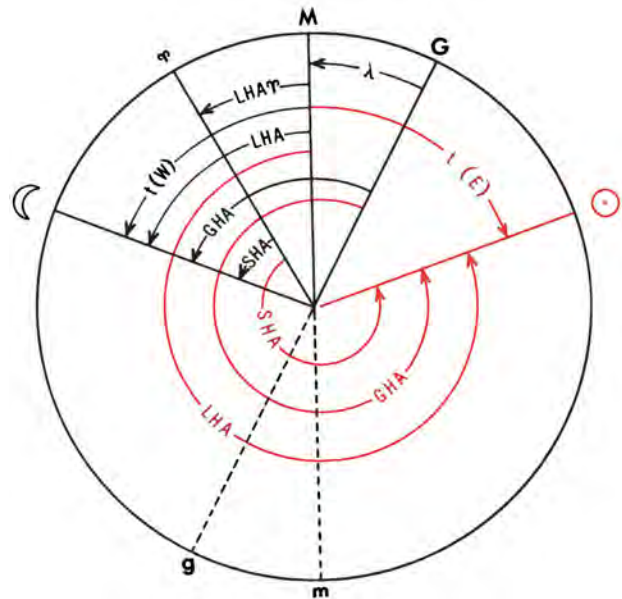
Figure 300. Time Diagram
