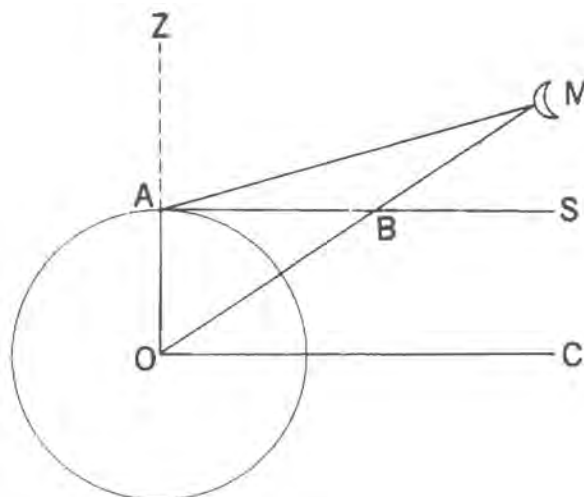
Figure 611. Geocentric parallax.
