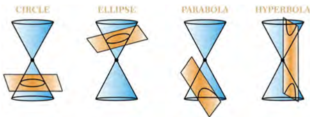
Figure 133a. Conic sections.
