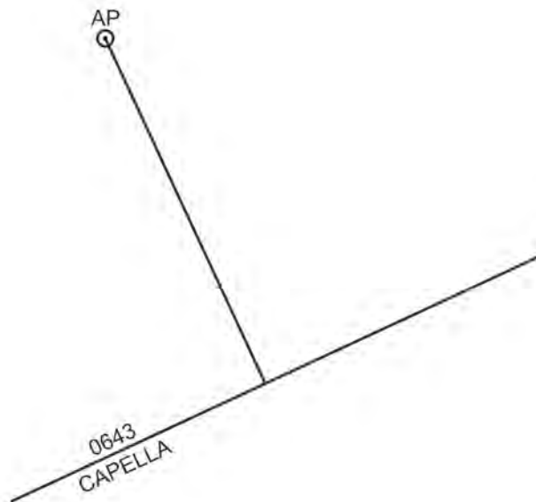
Figure 804. A line of position from observation of the star Capella at 0643
