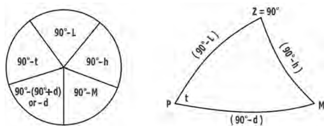
Figure 710. Circular parts diagram for astronomical triangle PMZ
