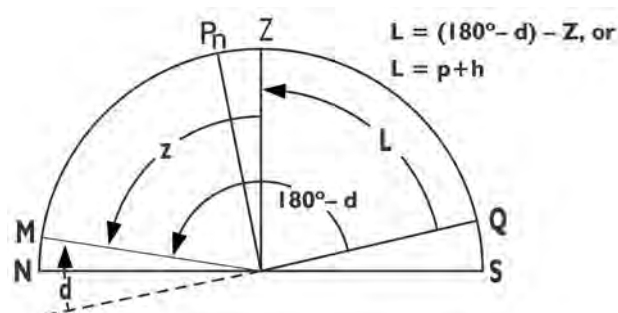
Figure 716h. Meridian altitude at lower transit.
