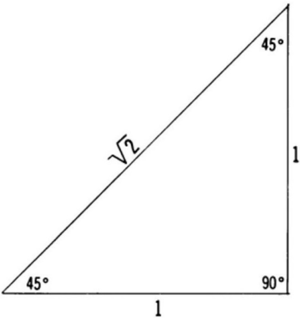
Figure 138d. Numerical relationship of sides of a 45°-45°-90° triangle.
