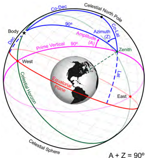
Figure 404. The amplitude angle (A) subtends the arc of the horizon between the body and the point where the prime vertical and the equator intersect the horizon. Note that it is the complement of the azimuth angle (Z).
