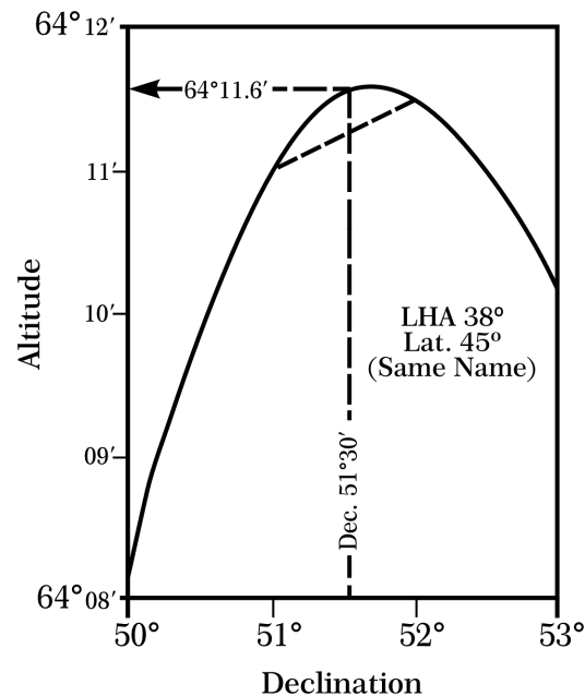
Figure 204b. Altitude curve.
