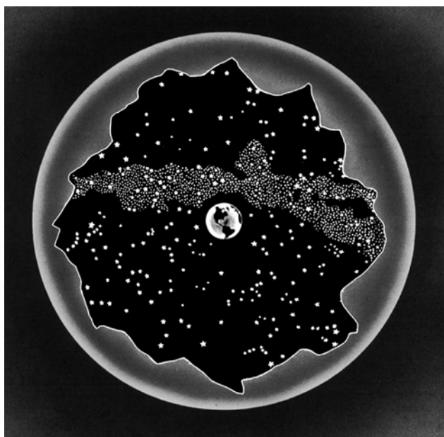
Figure G1a. The celestial sphere.
