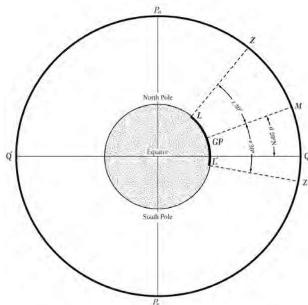
Figure 716a. Body on celestial meridian.
