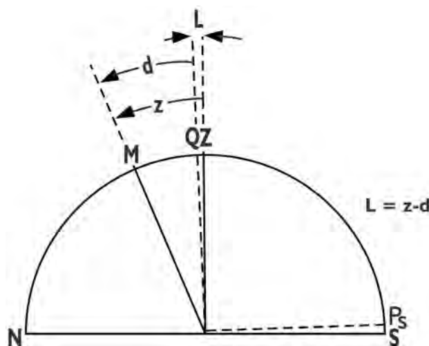
Figure 716q. Meridian transit in the vicinity of the equator.
