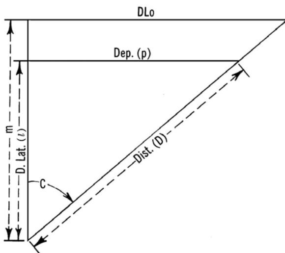
Figure 910a. Mercator and plane sailing relationship.
