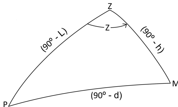
Figure 705b. Undivided astronomical triangle.
