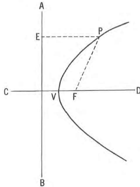
Figure 133c. A parabola.
