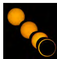
solar eclipse
