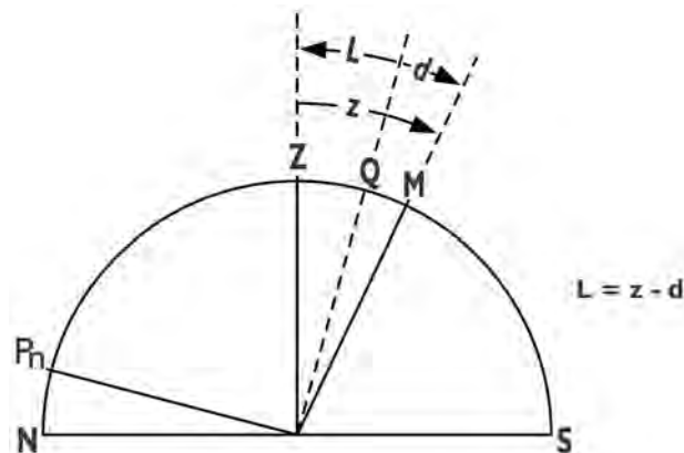
Figure 716d. Meridian altitude diagram.
