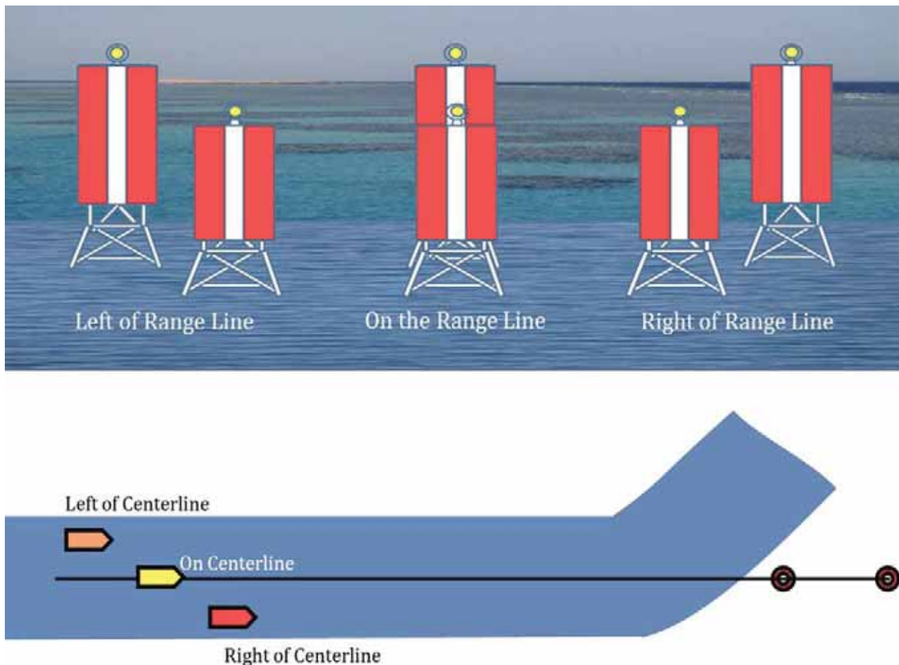
Figure 713. Example of Range Light aspects.
