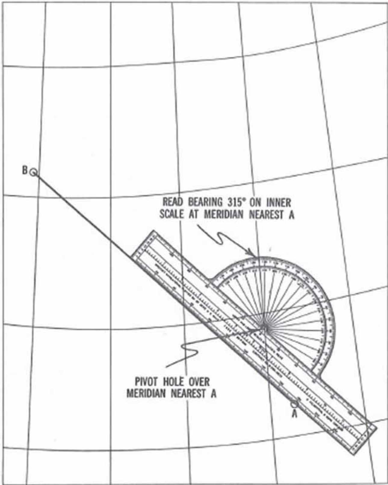
Figure 3319b. Measuring a bearing on a Lambert conformal chart. Note that the measurement is made at the meridian nearest the ship.
