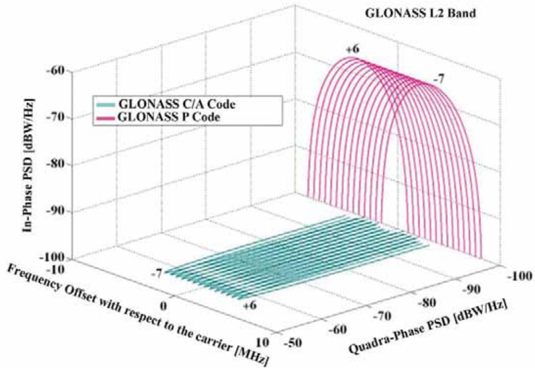
Figure 10a. Spectra of GLONASS signals in L2. Image courtesy of Dr. Jose Angel Avila Rodriguez.
