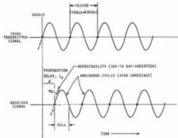
Figure 1614. Single tone time dissemination.
