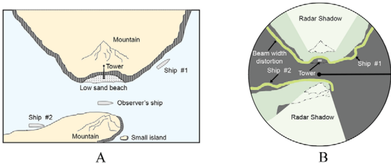
Figure 2309f. Distortion effects of radar shadow, beam width, and pulse length.
