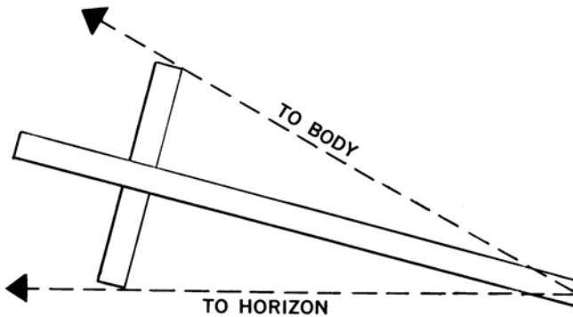
Figure 2808c. Improvised cross-staff.
