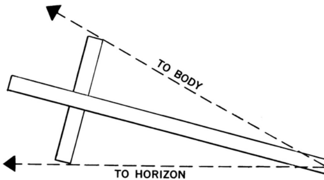
Figure 2808c. Improvised cross-staff.
