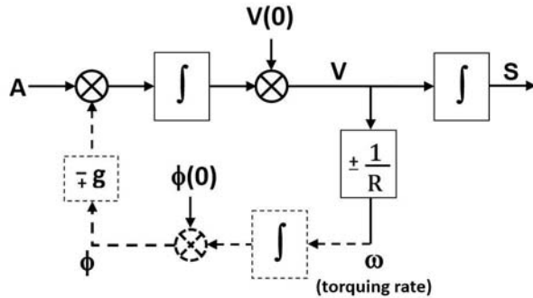
Figure 2018a. Block diagram of the Schuler loop.
