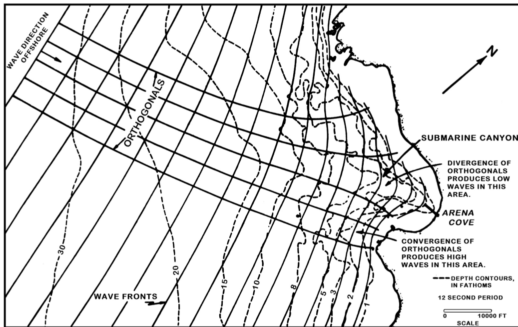
Figure 3715. The effect of bottom topography in causing wave convergence and wave divergence. Courtesy of Robert L. Wiegel, Council on Wave Research, University of California.
