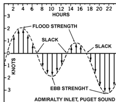
Figure 3515b. Reversing tidal current.
