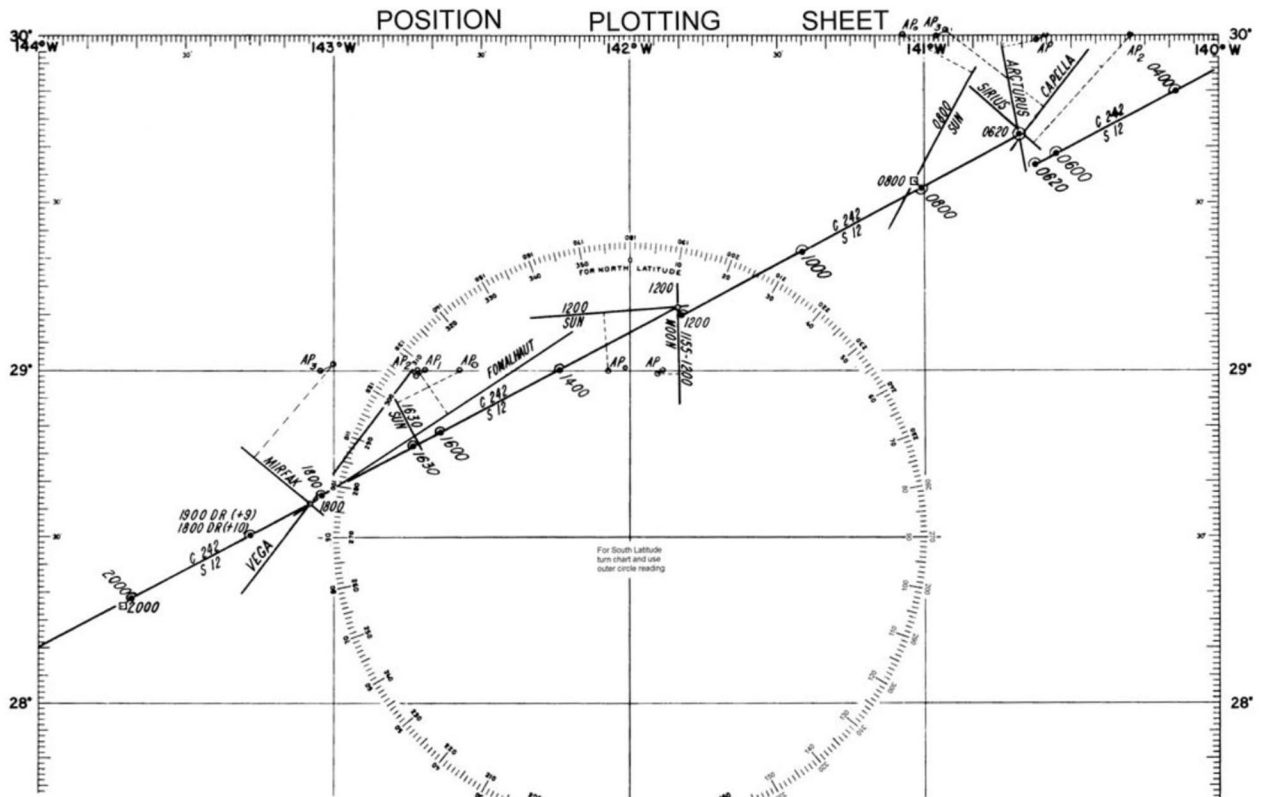
Figure 1913. Typical celestial plot at sea.
