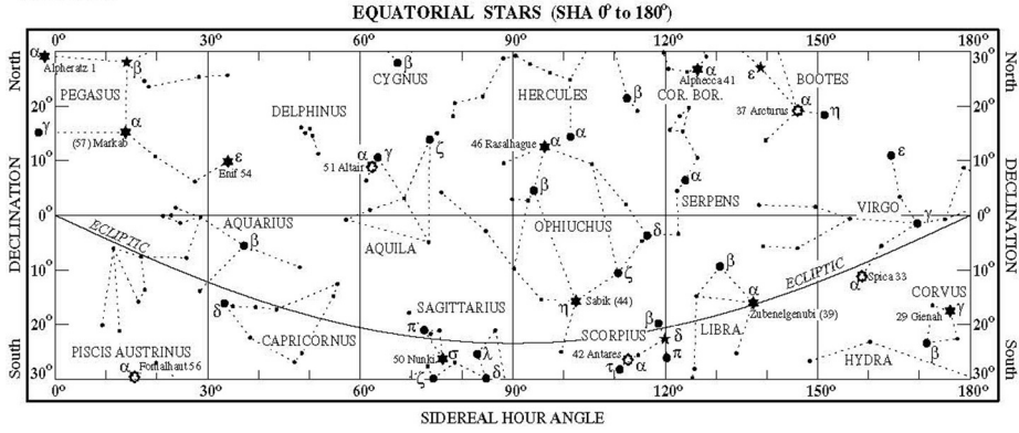
Figure 1334a. Star chart from Nautical Almanac.
