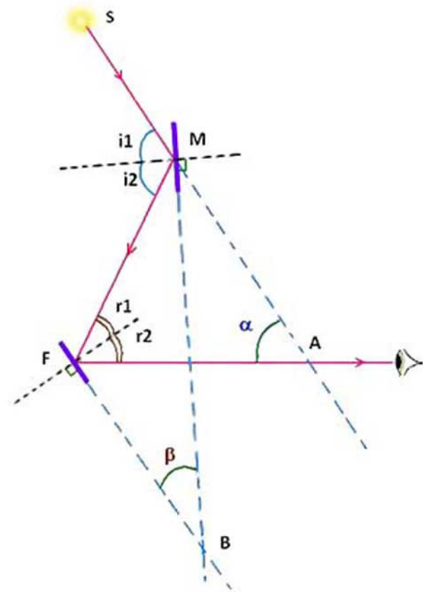
Figure 1401. Optical principle of the marine sextant.
